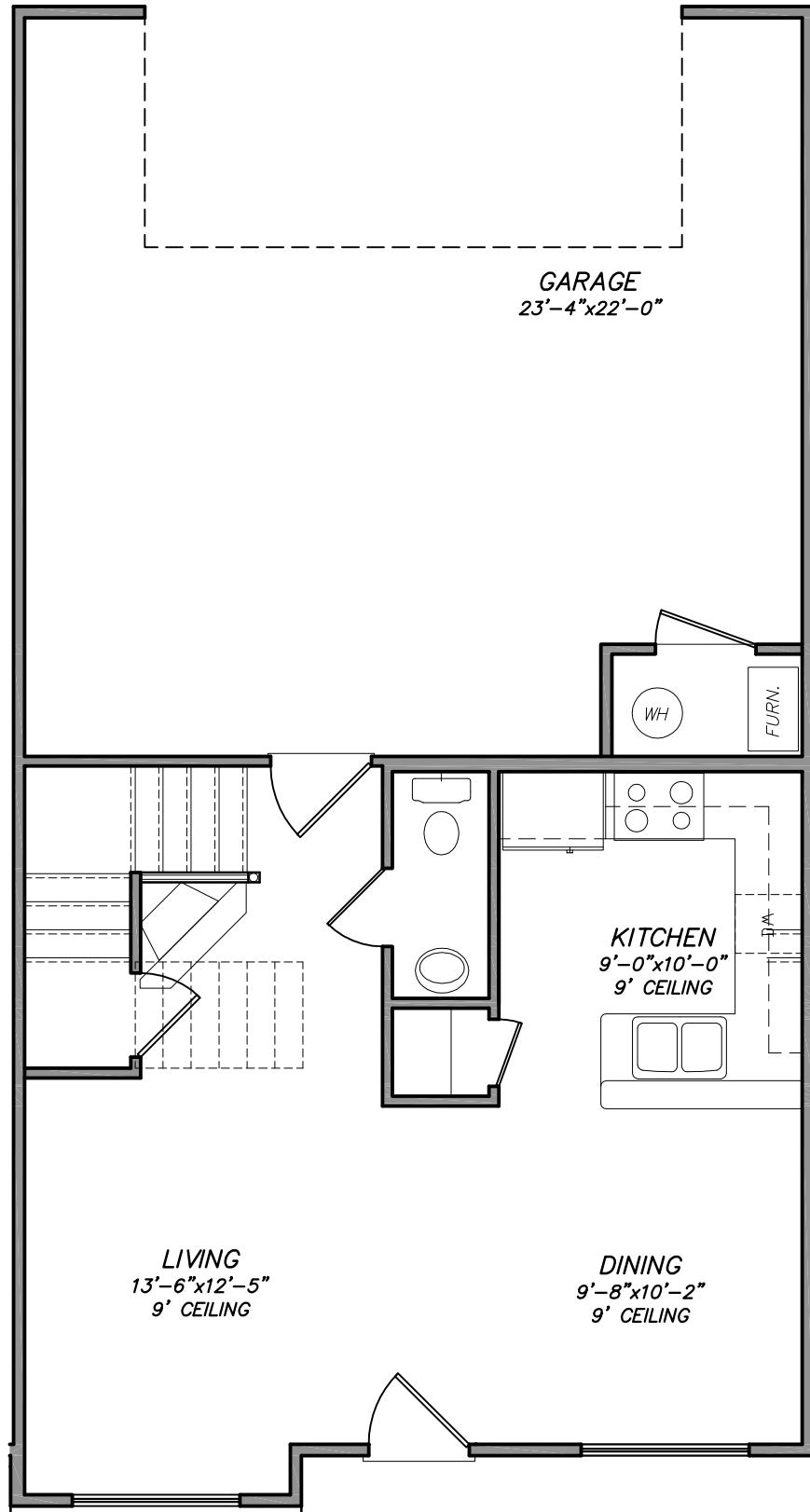
MAIN LEVEL FLOOR PLAN
